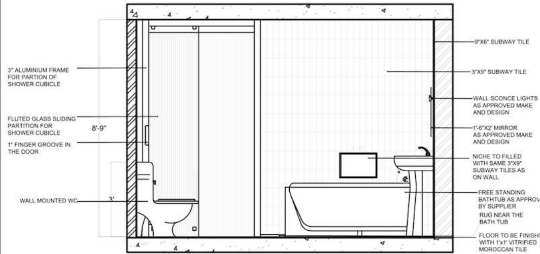
SECTIONAL ELEVATION C-C'
