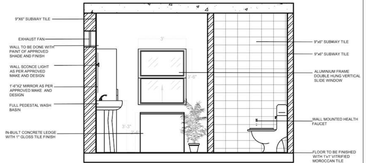
SECTIONAL ELEVATION D-D'
