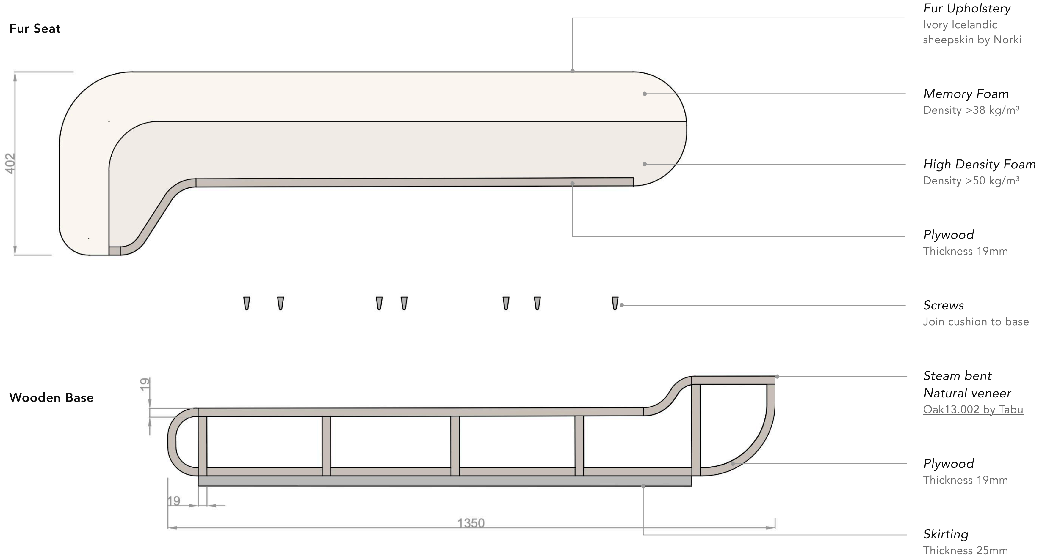
Sectional Elevation
