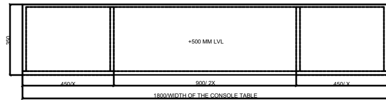
LAYOUT PLAN - UNDERCOUNTER UNIT
