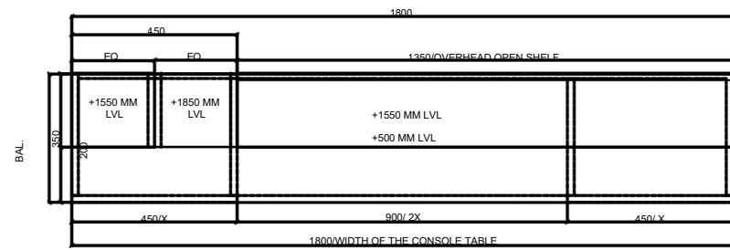
LAYOUT PLAN - COMBINED LCD UNIT
