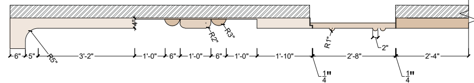
PLAN VIEW
