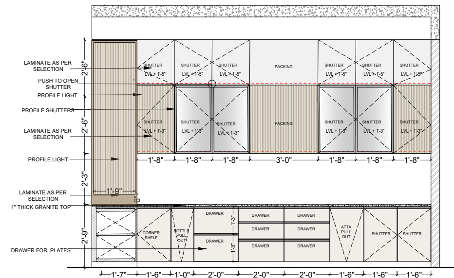
WALL ELEVATION A
