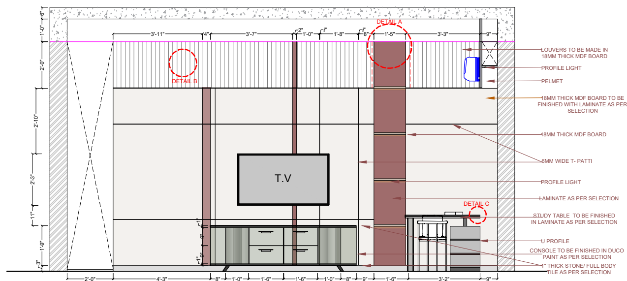
WALL ELEVATION B
