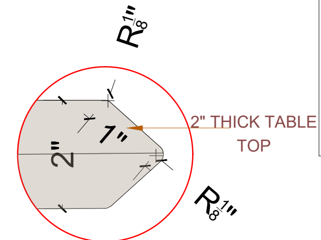
DETAIL C
