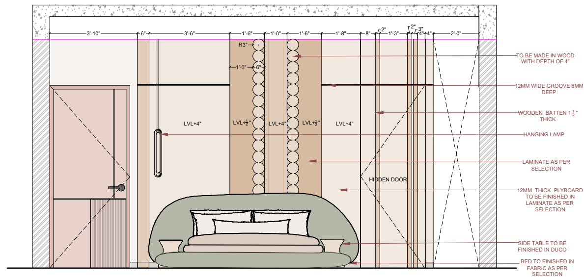
WALL ELEVATION A
