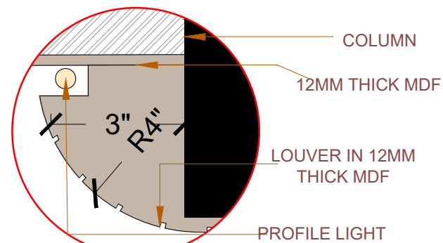
DETAIL A
