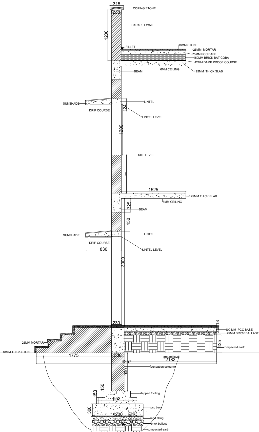
FOUNDATION AND STRUCTURE SECTION
