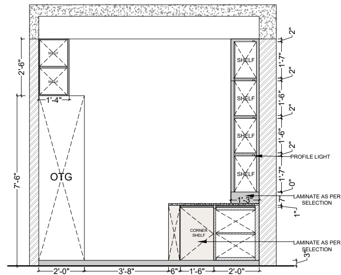
WALL ELEVATION C
