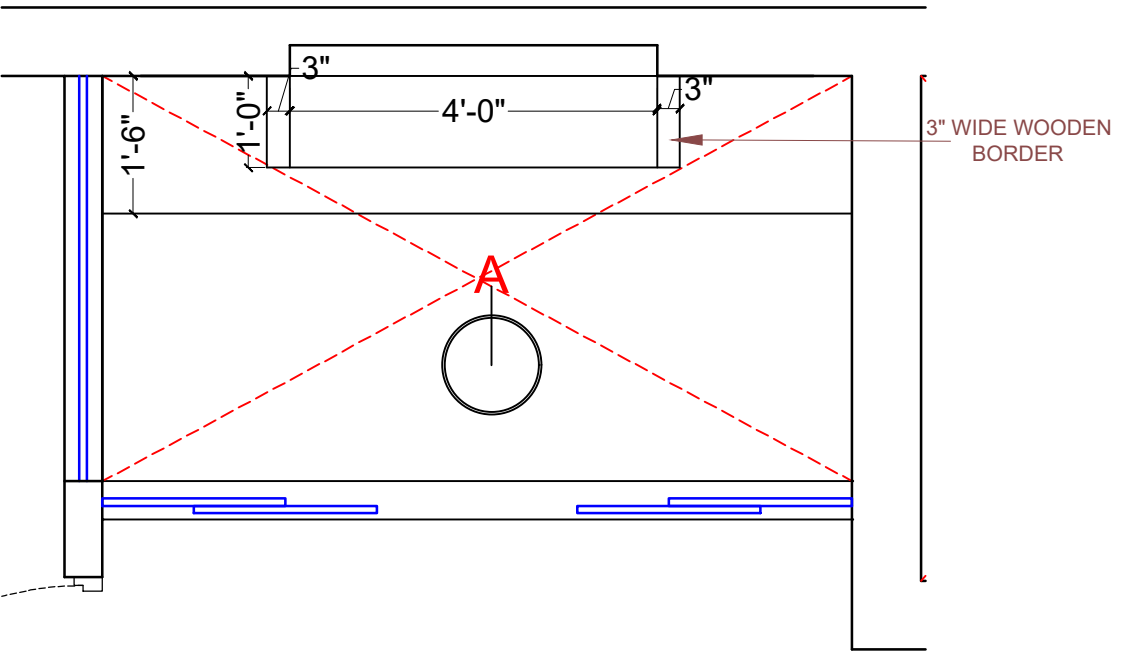
PLAN VIEW
