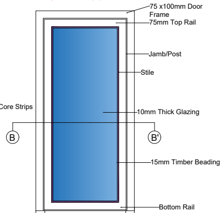
GLAZED DOOR
