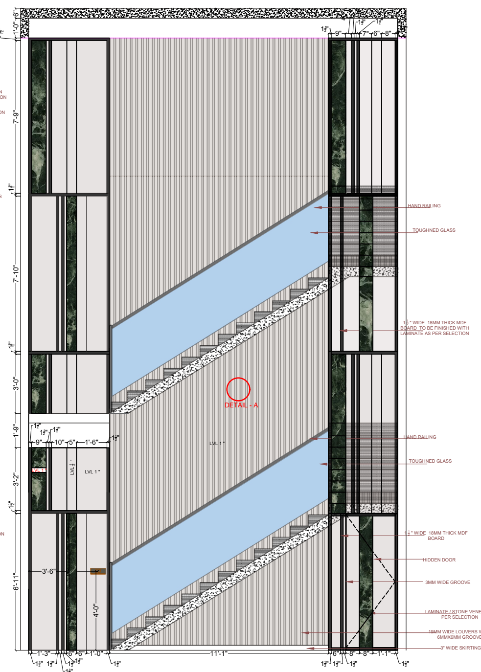
WALL ELEVATION - C
