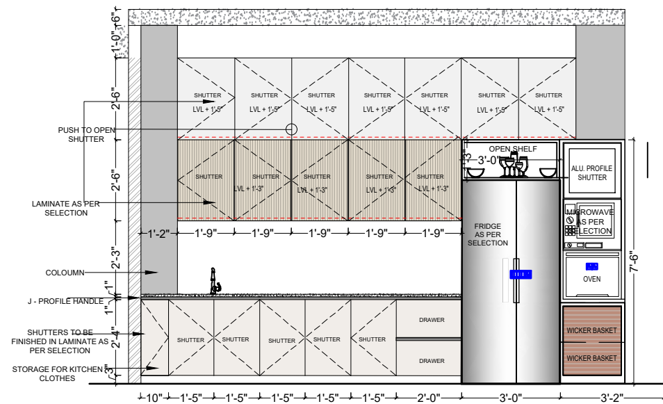
WALL ELEVATION B
