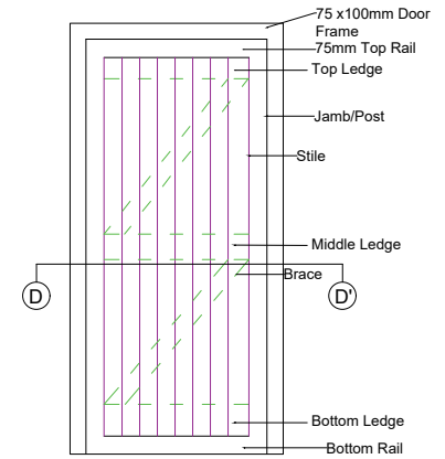
LEDGE, BATTENED, BRACED AND FRAMED DOOR
