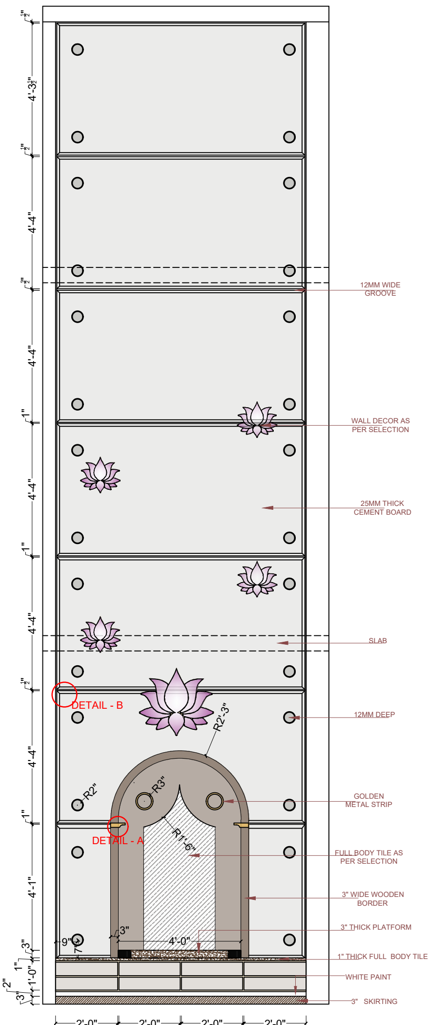
WALL ELEVATION - A
