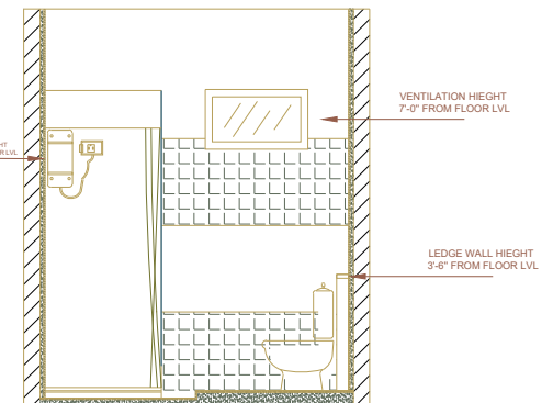
wall D
