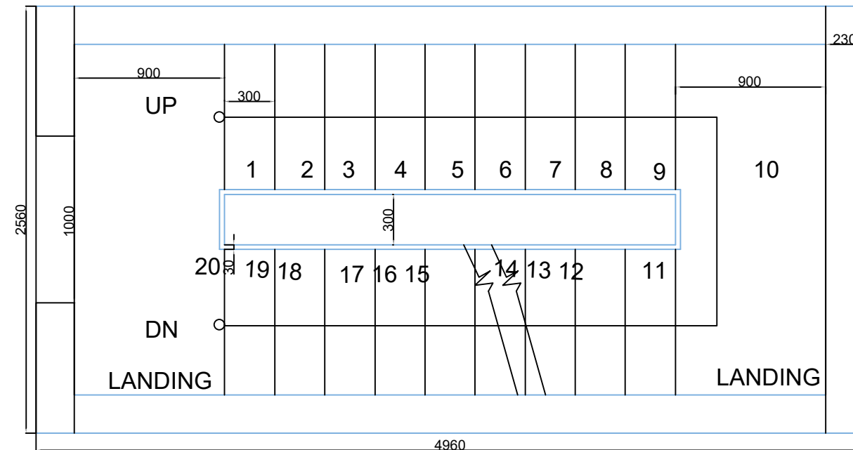
PLAN VIEW STAIRS
