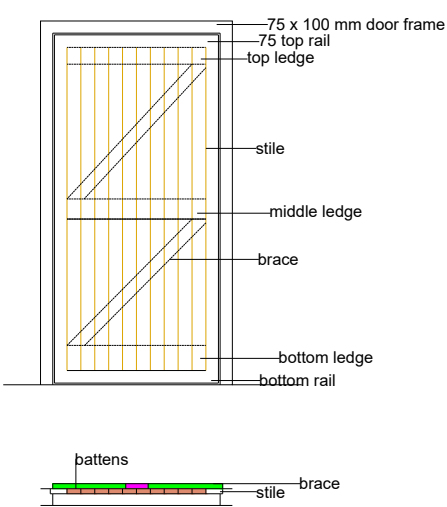
BATTENED ,LEDGED ,BRACED AND FRAMED DOOR
