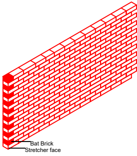
STRETCHER BOND
