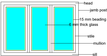
GLAZED OPENABLE WINDOW
