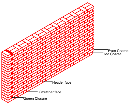
FLEMISH BOND
