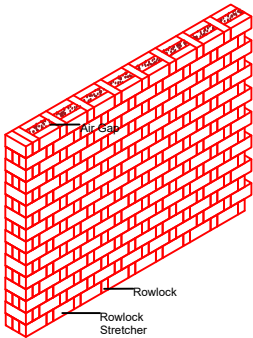
RAT TRAP BOND
