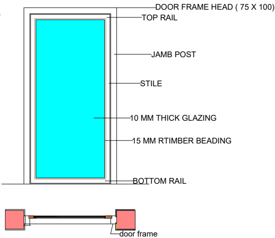
GLAZED DOOR
