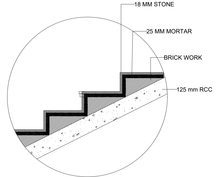
DETAIL 01
