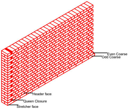
ENGLISH BOND
