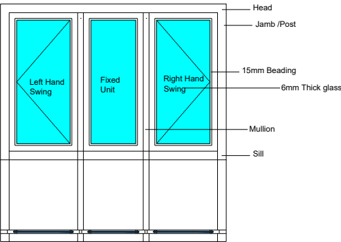
Casement Window
