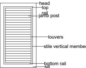
WOODEN LOUVER WINDOW
