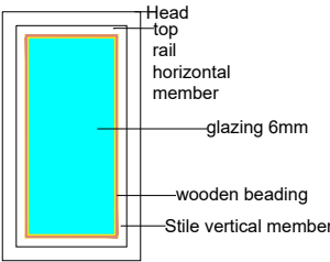
GLAZED FIXED WINDOW
